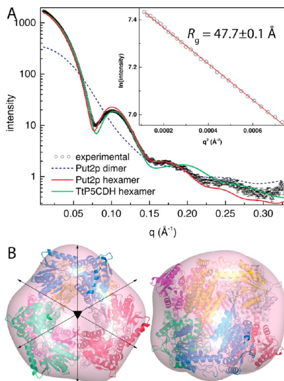
Figure 5. SAXS analyses of Put2p. (A) Experimental and calculated SAXS curves. The inset shows a Guinier plot spanning the qR_g range of 0.508–1.29. The linear fit of the Guinier plot has an R^2 of 0.9995. (B) Superposition of the SAXS shape reconstruction envelope and the Put2p hexamer generated from crystallographic symmetry. Two orthogonal views are shown.
