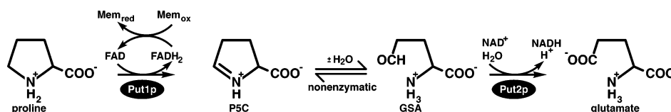
Figure 1. Reactions catalyzed by the yeast proline catabolic enzymes Put1p and Put2p.
