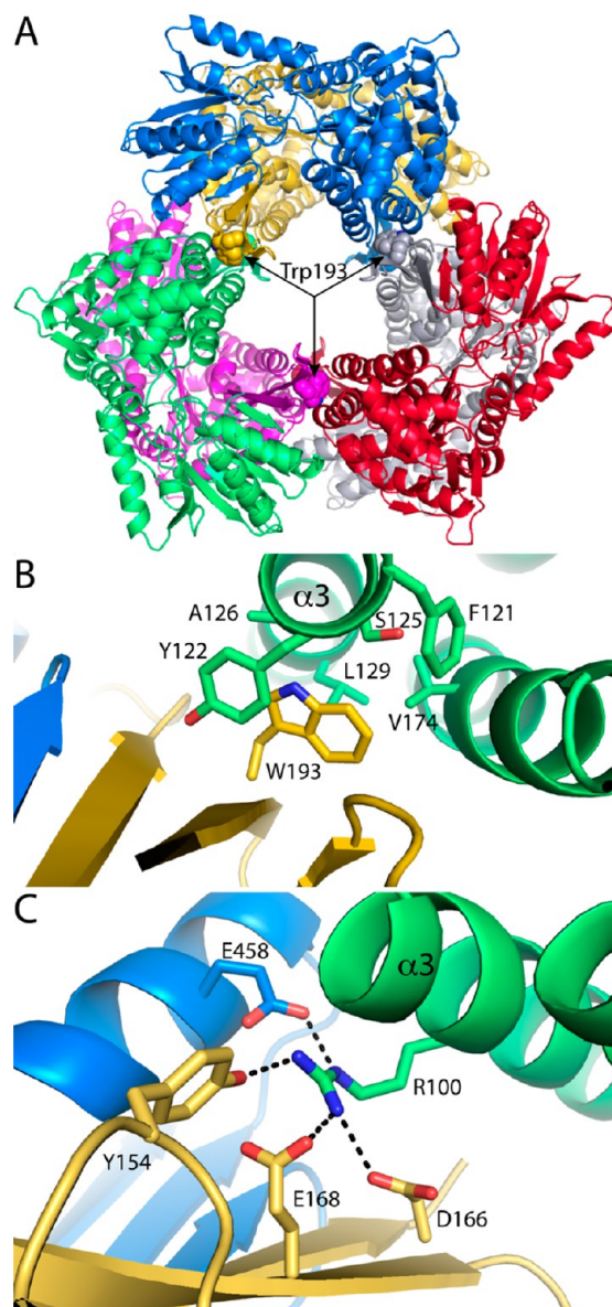
Figure 6. Hexamerization hot spots of Put2p and TtP5CDH. (A) Put2p hexamer viewed down the 3-fold axis, showing the location of the hot spot centered on Trp193 (shown as spheres). The six chains have different colors. (B) Close-up view of the environment around Trp193 of Put2p. The chains are colored as in panel A. (C) Hot spot of TtP5CDH, which is centered on Arg100 of \alpha 3 . The chains are colored as in panel A.
