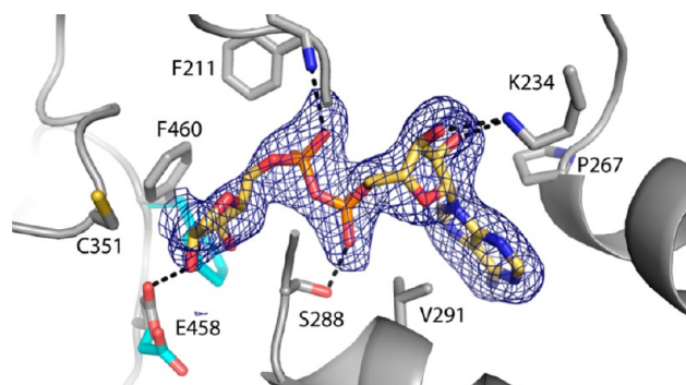
Figure 4. Electron density and interactions for NAD + bound to Put2p. The cage represents a simulated annealing \sigma_A -weighted F_o - F_c omit map contoured at 3.0\sigma . The conformations of Glu458 and Phe460 prior to NAD + binding are colored cyan.
