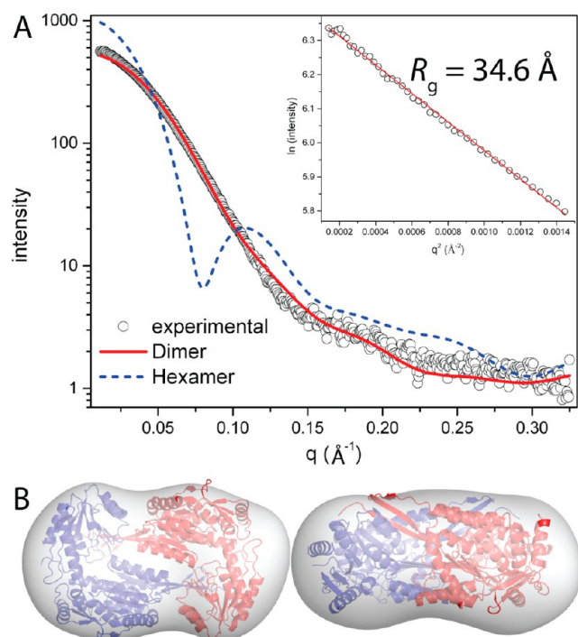
Figure 8. SAXS analysis of W193A. (A) Experimental and calculated SAXS curves. The inset shows a Guinier plot spanning the qR_g range of 0.346–1.34. The linear fit of the Guinier plot has an R^2 of 0.997. (B) Superposition of the SAXS shape reconstruction envelope and the Put2p dimer from the asymmetric unit. Two orthogonal views are shown.
