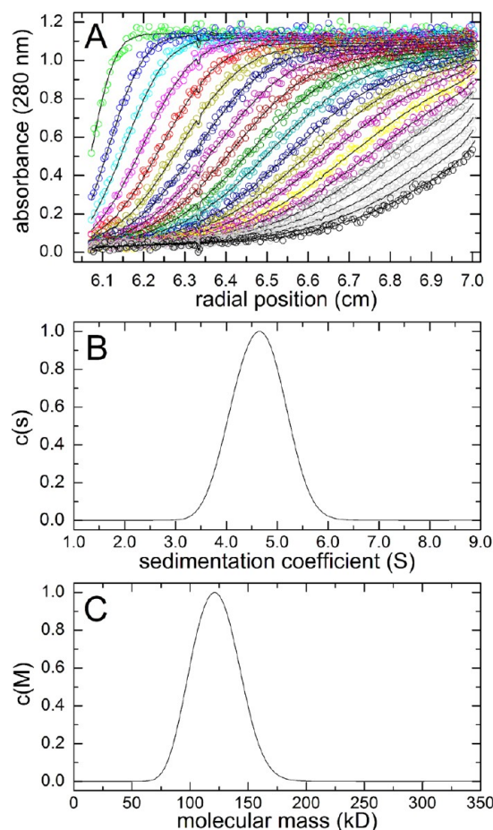
Figure 7. Sedimentation velocity analysis of W193A. (A) Selected velocity profiles (circles) and optimal least-squares fits. (B) Sedimentation coefficient distribution. (C) Molecular mass distribution.
