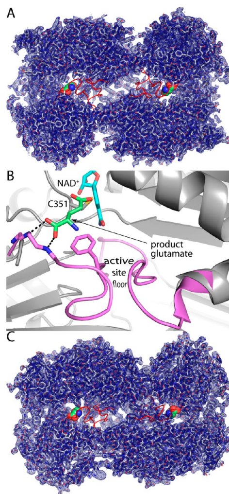
Figure 3. Electron density evidence for disorder in the aldehyde-binding loops of Put2p and HsP5CDH. (A) Put2p dimer with 2F_o - F_c electron density ( 1.0\sigma ). The red sections represent the aldehyde-binding loops transplanted from MmP5CDH. The green spheres represent the product glutamate bound to MmP5CDH (PDB entry 3v9k). (B) Close-up view of the expected conformation of the aldehyde-binding loop in Put2p. Put2p is colored gray. The aldehyde-binding loop (pink), bound glutamate ligand (green), and NAD + of MmP5CDH have been fit onto Put2p to guide the eye. (C) Dimer of monoclinic HsP5CDH with 2F_o - F_c electron density ( 1.0\sigma ). The red sections represent the aldehyde-binding loop of MmP5CDH, which is disordered in the monoclinic crystal form of HsP5CDH. The green spheres represent the product glutamate bound to MmP5CDH.
