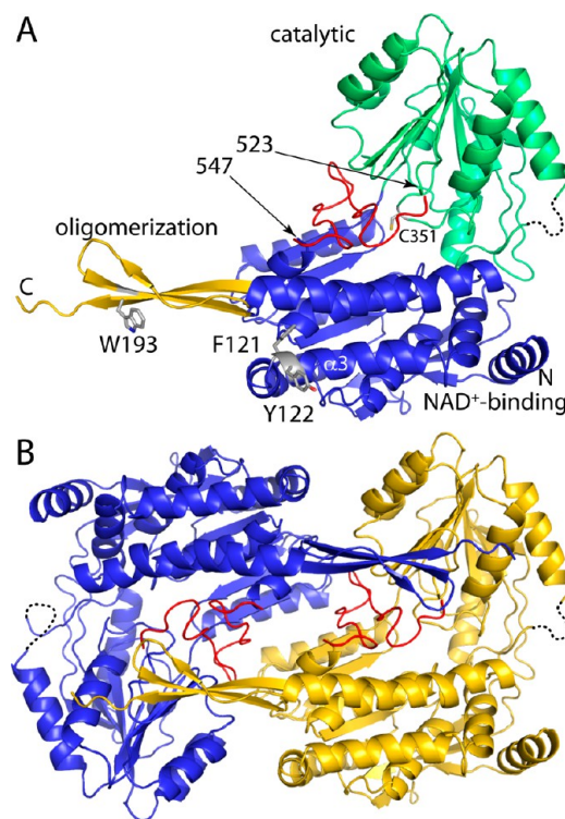
Figure 2. Structure of Put2p. (A) Protomer with the catalytic domain colored green, the \text{NAD}^+ -binding domain blue, and the oligomerization domain gold. The red sections represent the aldehyde-binding loop (transplanted from a MmP5CDH structure), which is disordered in Put2p. Selected side chains of the hexamerization hot spot are colored gray (Trp193, Phe121, and Tyr122). (B) Structure of the Put2p dimer in the asymmetric unit. The two protomers are colored blue and gold. Red sections represent the aldehyde-binding loop, which is disordered in Put2p.
